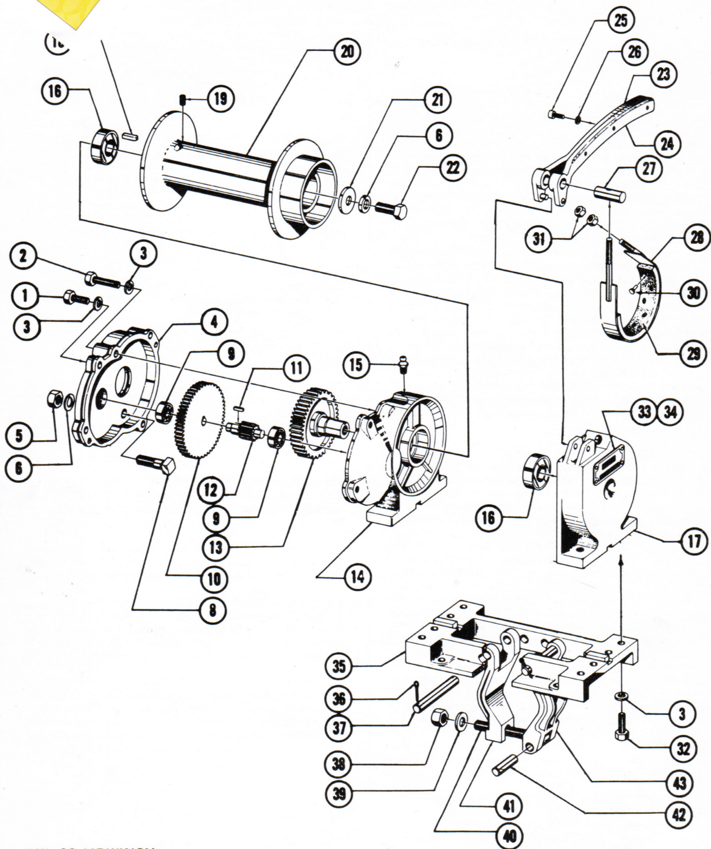
AW-80 AIRWINCH EXPLODED VIEW
